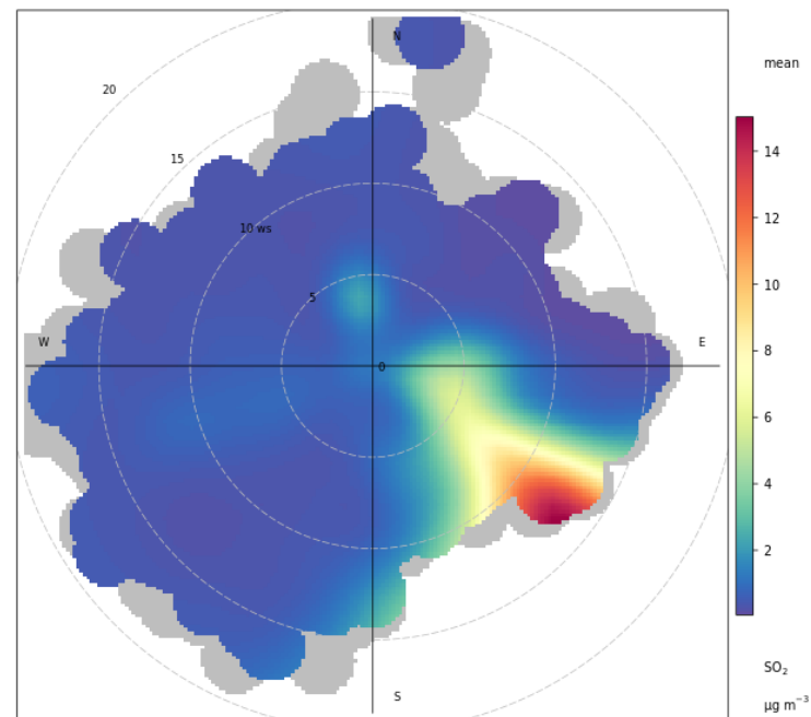
Polar plot of SO 2 at Falkirk Grangemouth MC mean for the period 2020 to 2024
