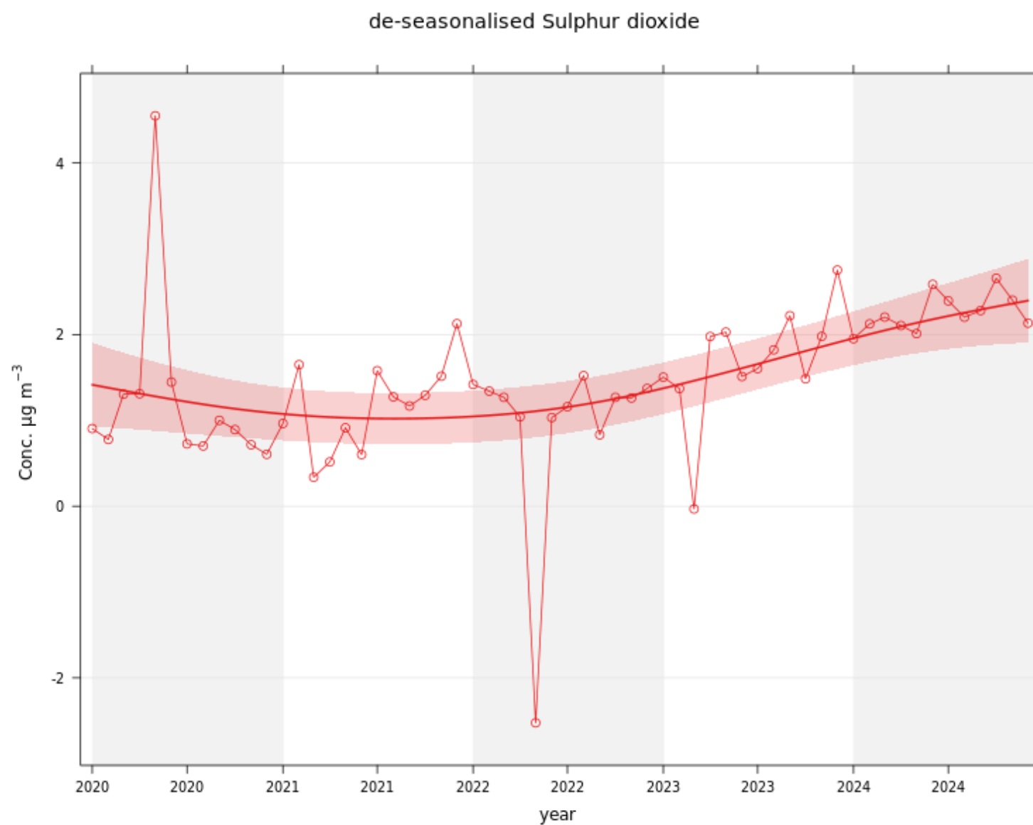
Figure 26 – A10 Grangemouth Municipal Chambers Long Term SO 2 Concentrations
