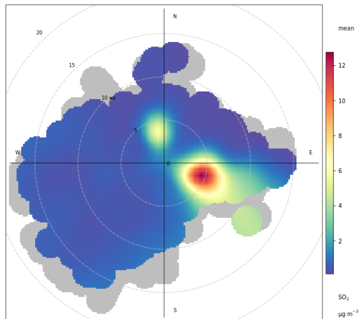
Polar plot of SO 2 at Falkirk Grangemouth MC mean for the period 2024 to 2024
