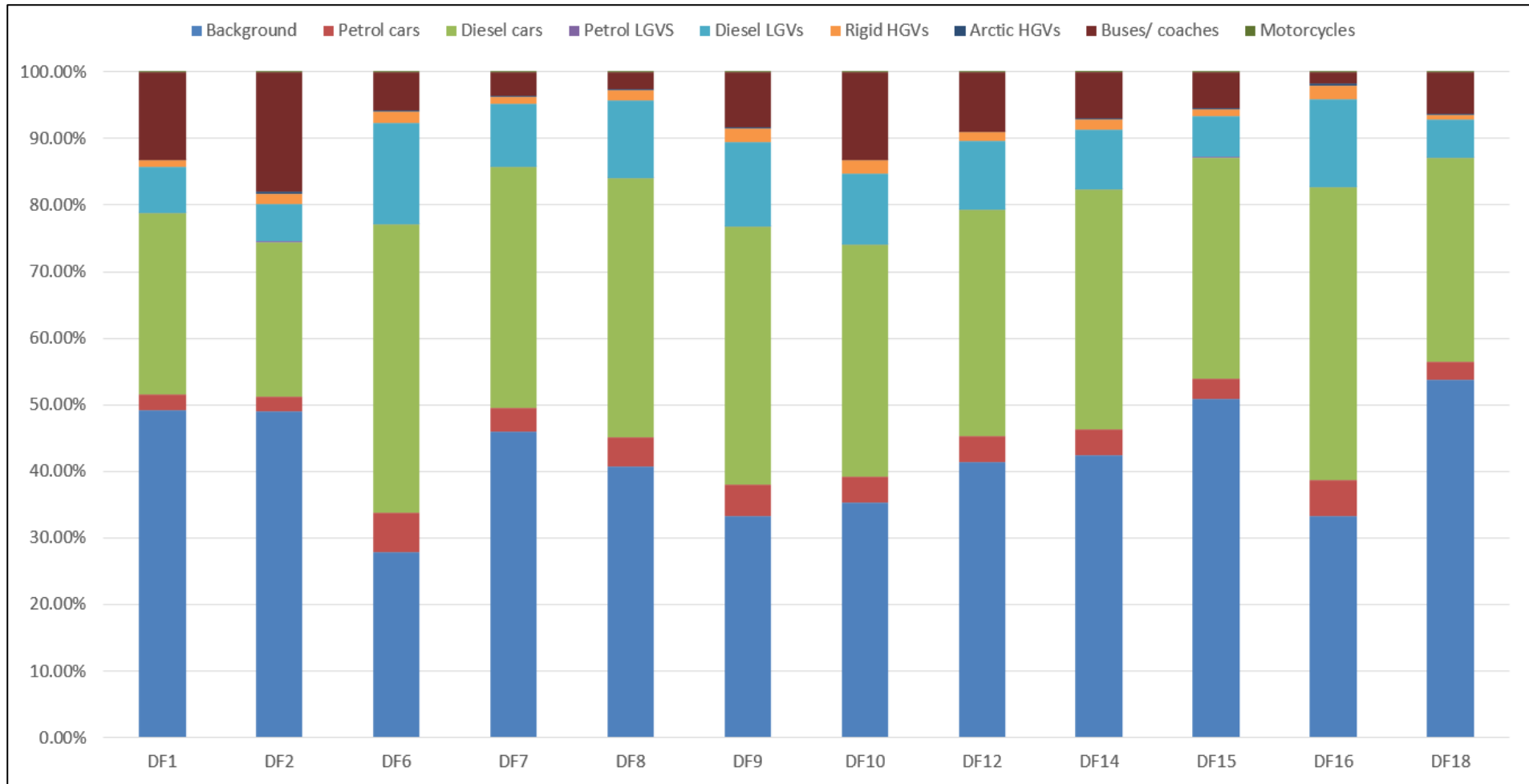
Figure 5: Stacked bar chart showing NOx source apportionment for all road transport and background for monitoring locations within Blackpool AQMA (%), for the baseline fleet, 2022
