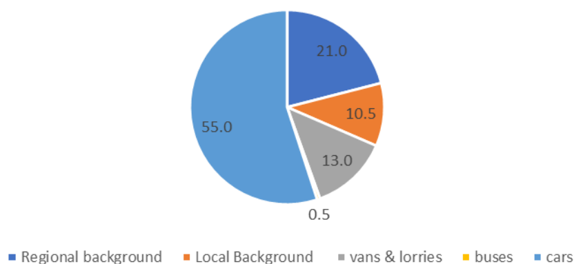
AQMA No 1/2011 Stragglethorpe Road Source Apportionment - Percentage Contribution
